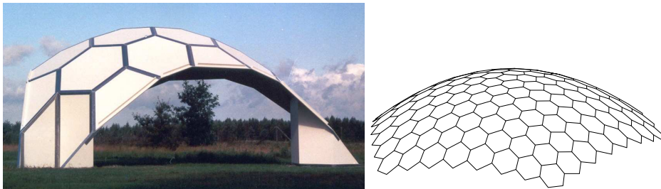
Fig. 3. Left: Plate shell structure consisting of plates primarily subjected to in-plane shear and normal forces (Full scale model, SBI Hørsholm). Right: Principle layout for a load carrying faceted shell structure of glass.
