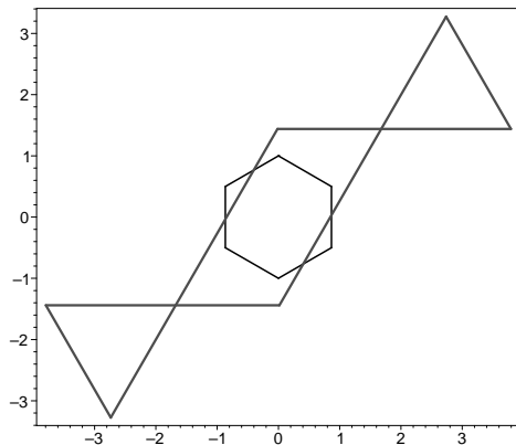
Fig. 8. The limit shape (thick polygon) associated with the star defined by the regular hexagon for the surface (39).
