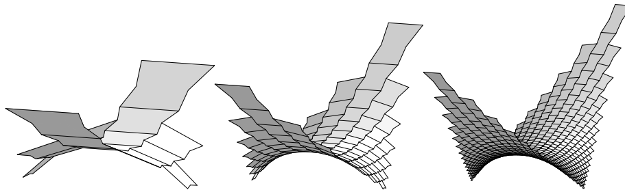
Fig. 11. Primal tangent meshes of a ruled quadric for three different values of h .
