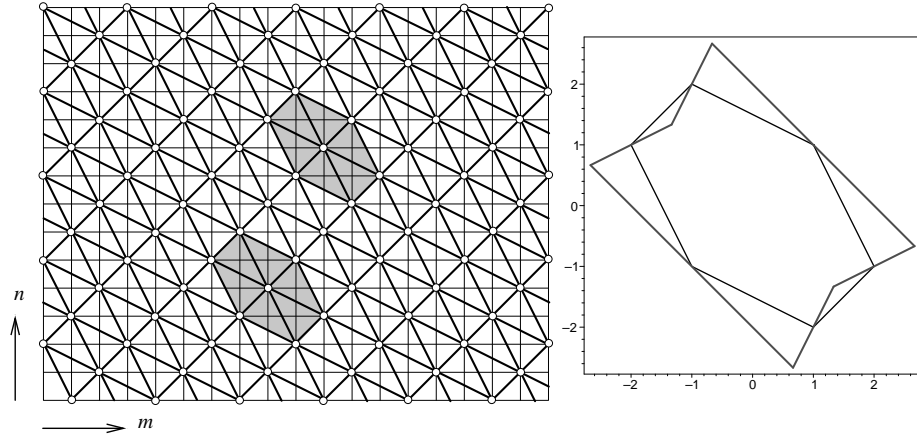
Fig. 9. Left: Pattern for producing the dual mesh from the dual surface. The vertical and horizontal lines represent the grid of asymptotic lines, while the circles indicate which points should be sampled. Right: The limit shape (thick curve) of the star defined by the thin polygon, which corresponds to the hexagons shown in the left figure.
