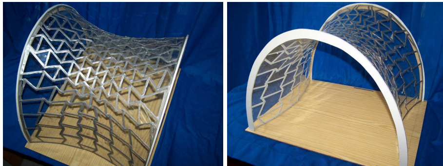
Fig. 7. Example 4. Non-convex mesh with piecewise linear support function which approximates a segment of a one-sheeted hyperboloid. The mesh has 169 facets.
