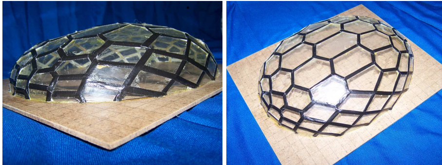
Fig. 6. Example 3. Convex mesh with piecewise linear support function which approximates a segment of an ellipsoid. The mesh consists of 90 facets.
