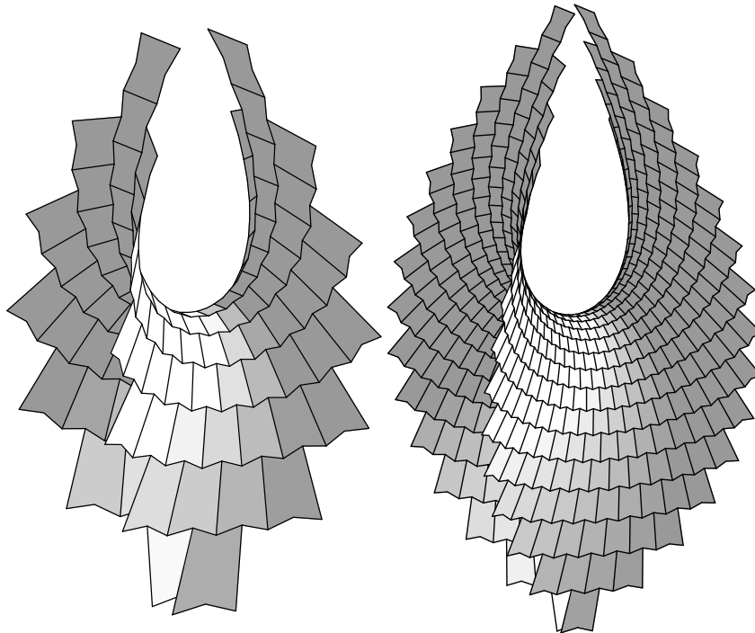
Fig. 10. Primal tangent meshes of the Enneper surface for values h = 0.081 (left) and h = 0.039 (right).
