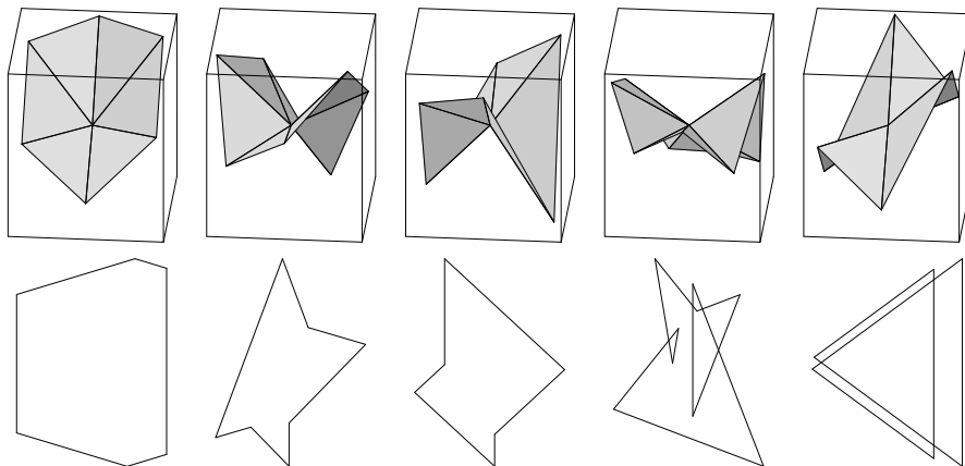
Fig. 5. Stars of vertices of the dual mesh and the associated quasi-convex polygons of the primal mesh. From left to right: convex, simple; non-convex, simple ( 2\times ); non-convex, non-simple ( 2\times ).
