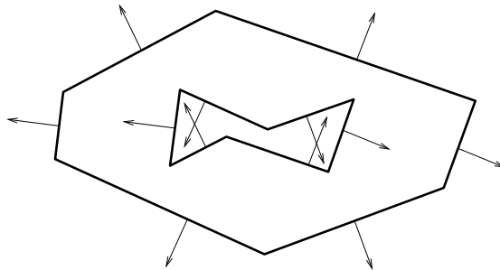
Fig. 4. Quasi-convex polygons as offsets of convex polygons.
