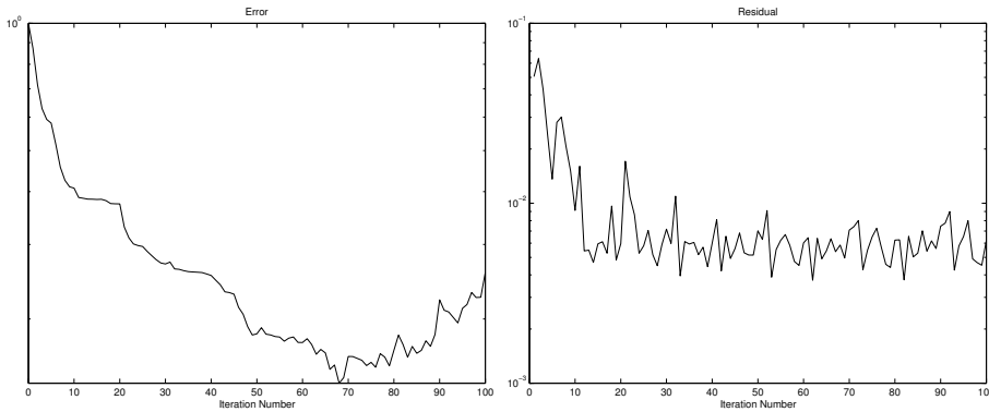
FIG. 5.8. Semi-logarithmic plot of error (left) and residual (right) vs. iteration number in the second example, \delta = 1\%
