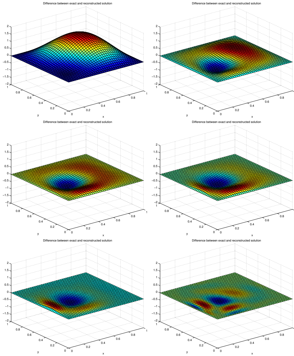
FIG. 5.6. Difference \hat{q} - q_n in the first examples at iterates 1, 2, 3, 5, 10, and 100.
