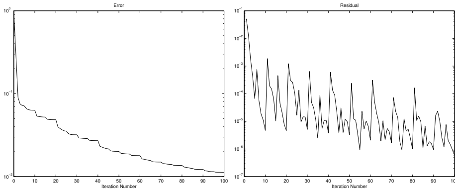
FIG. 5.7. Semi-logarithmic plot of error (left) and residual (right) vs. iteration number in the second example, \delta = 0
